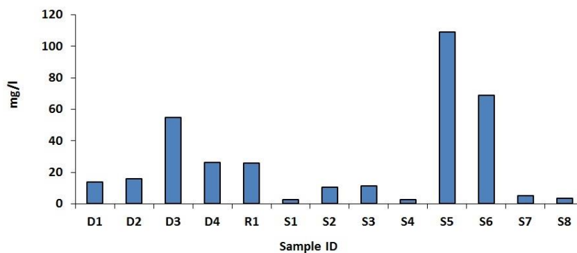
Figure 4.18. The concentration of sodium ions in water samples
