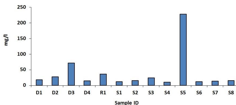
Figure 4.26. The concentration of chloride ions in water samples
