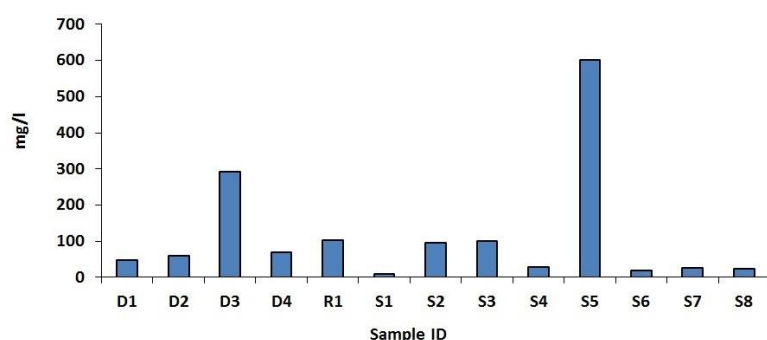
Figure 4.28. Concentration of nitrate ions in water samples
