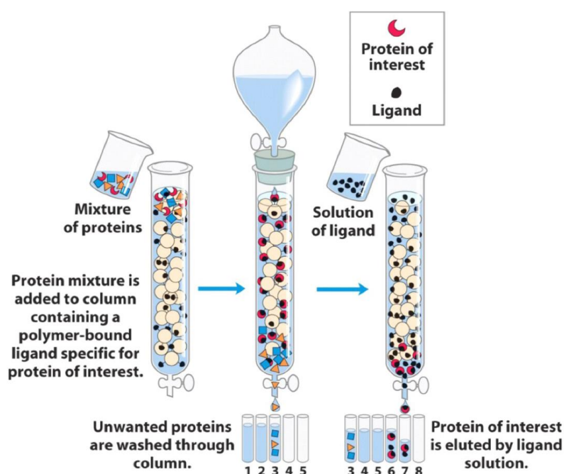
Figure 3.1. Protein purification steps by affinity chromatography (Lehninger 2008)
