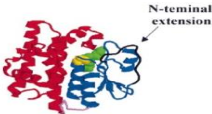
Figure 1.8. Three-dimensional structure of human omega class GST. The N-terminal domain 1 is coloured blue, while the C-terminal domain 2 is red. Catalytically essential cysteine residue is shown as space filling model (sheehan et al. 2001)
