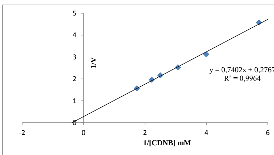
Figure 4.9. The Linweaver-Burk reciprocal plot for the CDNB substrate. Different concentration of the CDNB substrate for GST Rat's erythrocytes enzyme used, in order to find the maximum velocity of the enzyme and the Michealis-Menten constant of the substrate
