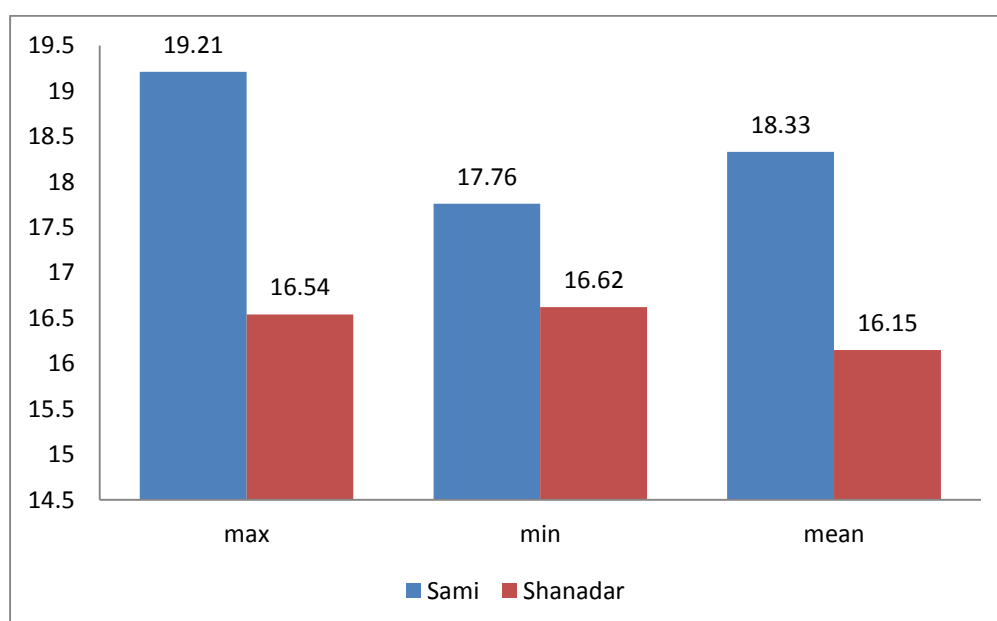
Figure 19. Mean with minimum and maximum acidity at 8 stations in Sami Abdurrahman with Shanadar Park and its tributaries during the studied period
