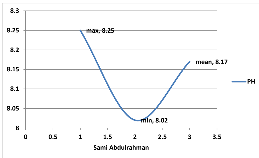
Figure 22. Mean with minimum and maximum pH at 4 stations in Sami Abdulrahman Park and its tributaries during the studied period
