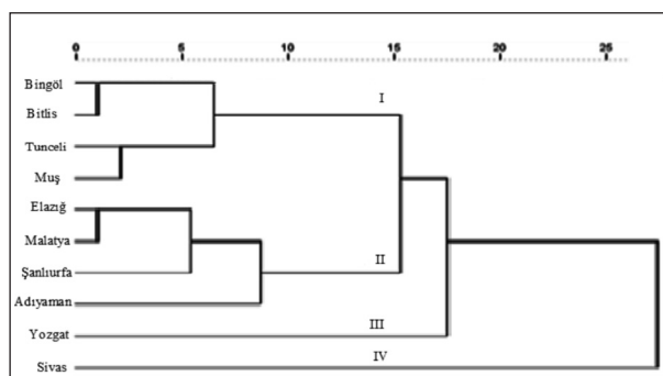
Figure 2. Average-linkage dendrogram of the ten Hypericum scabrum populations resulting from the cluster analysis of the calli essential oil components. Chemotype I (Limonene / Germacrene D), Chemotype II ( \alpha -pinene), Chemotype III ( \beta -ocimene) and Chemotype IV ( \beta -pinene / \alpha -pinene).
