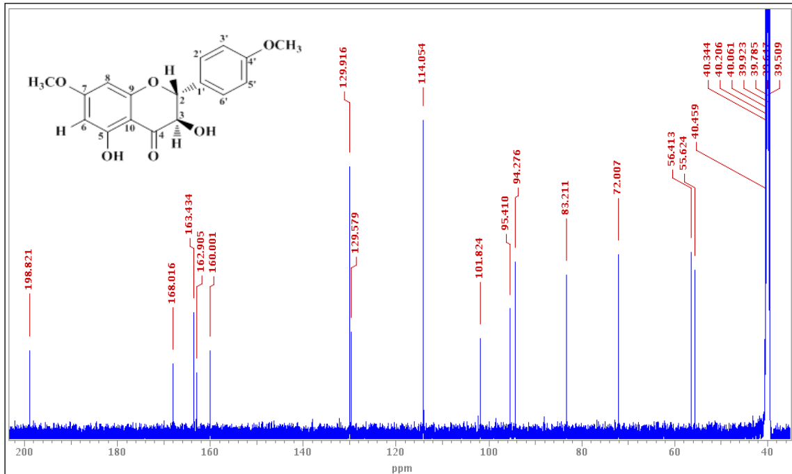
Şekil 4.45. (2R,3R)-(+)-dihidrokamferol-7,4'-dimetileter (5) bileşğinin ^{13}\text{C-NMR} spektrumu ( ^{13}\text{C} : 125 MHz; \text{DMSO-}d_6 )
