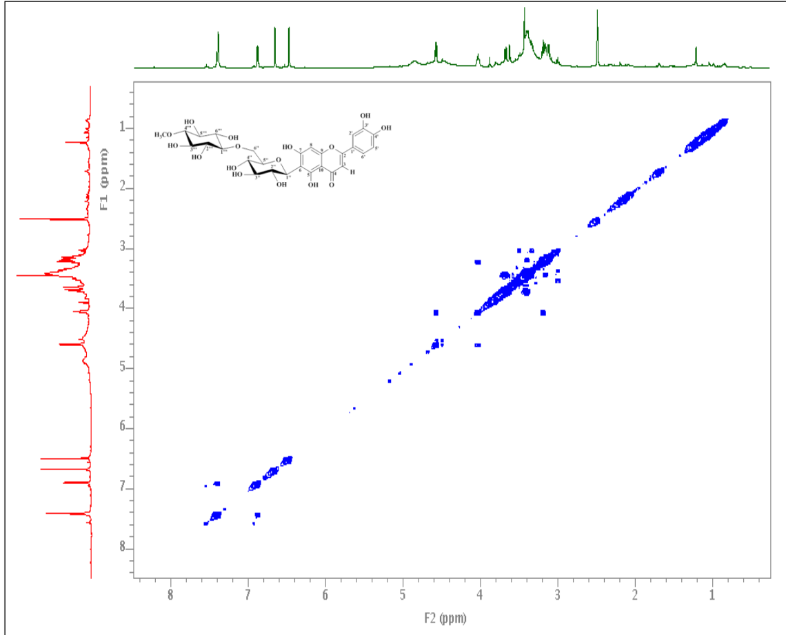
Şekil 4.26. Homoorientin-6''-4- O -metil- myo -inositol (2) bileşiginin ^1\text{H} - ^1\text{H} -gCOSY-NMR spektrumu ( ^1\text{H} : 600 MHz; \text{DMSO}-d_6 )
