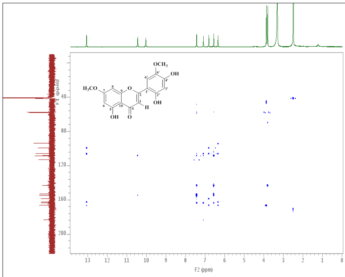
Şekil 4.13. 7,5'-dimetoksiisoeugenin (1) ^1\text{H} - ^{13}\text{C} -gHMBC-NMR spektrumu ( ^1\text{H} : 600 MHz; ^{13}\text{C} : 125 MHz; \text{DMSO-}d_6 )
